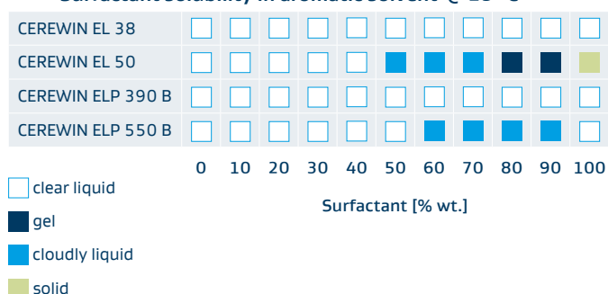
Surfactant solubility in aromatic solvent @ 25 °C
