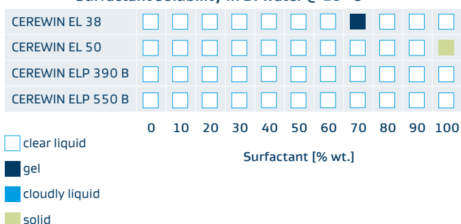
Surfactant solubility in DI water @ 25 °C
